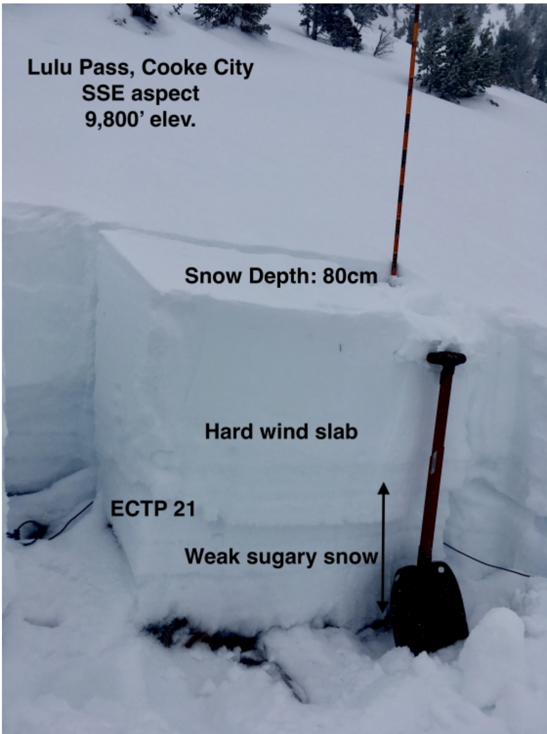
Near Cooke City, a poor snowpack structure has been found and produced avalanches on east, south and west aspects, and makes large avalanches possible to trigger. Photo: GNFAAC
